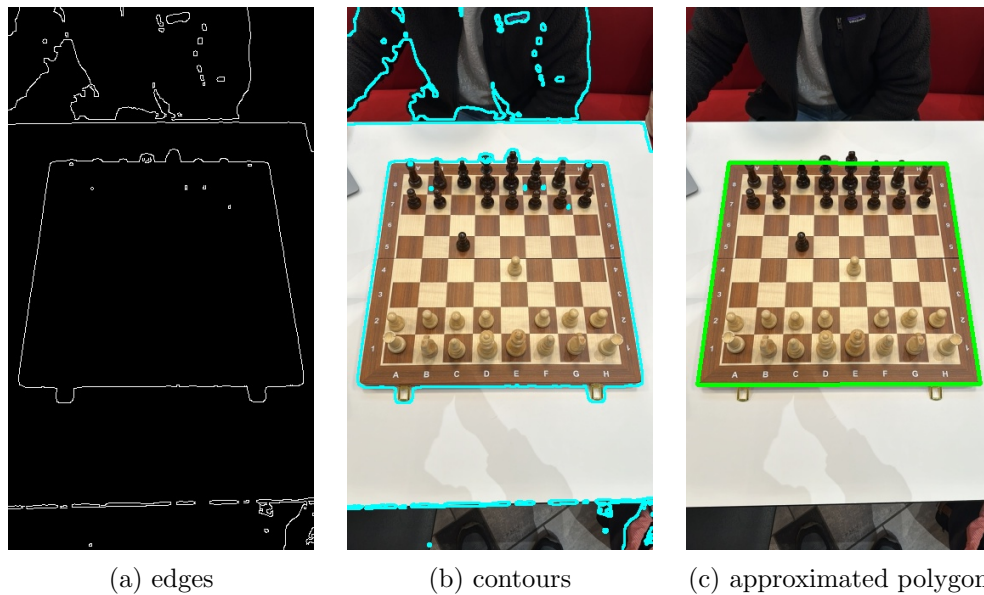
Figure 11: Steps from edge detection to board corners
