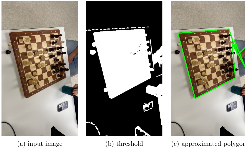
Figure 16: Failure to detect chessboard in image of first dataset due to table corner too close to the chessboard
