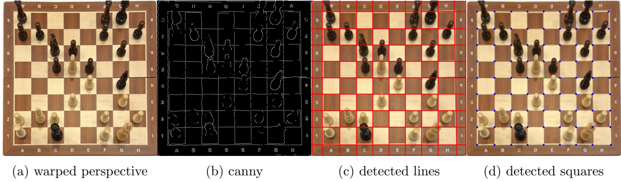
Figure 12: Steps to detect squares from board image
