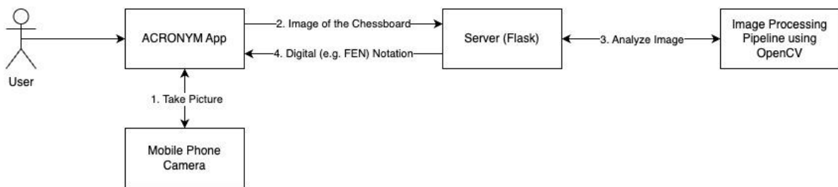
Figure 2: System Architecture and Interaction Diagram
