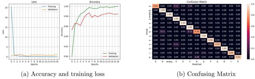
Figure 23: Results of training CNN classifier with additional random positions
