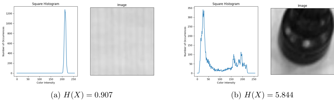
Figure 13: Histograms of grayscale squares
