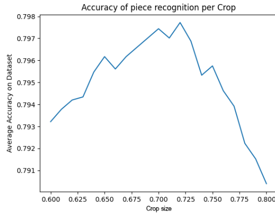
Figure 19: Accuracy of different amounts of cropping before calculating color average
