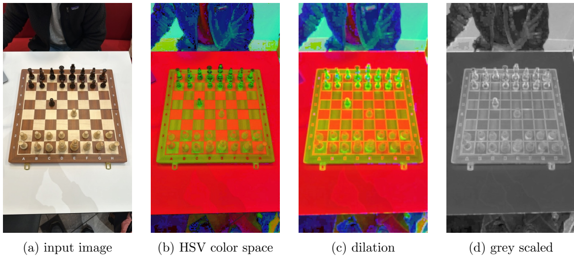
Figure 9: HSV dilation process
