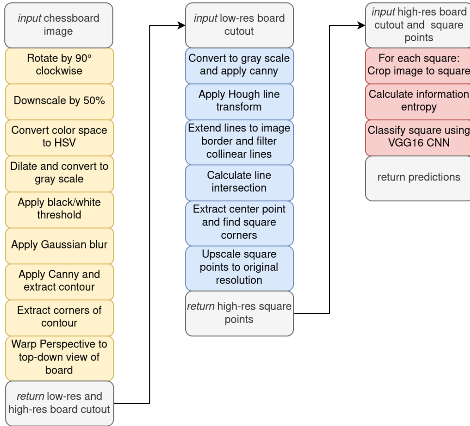
Figure 7: Overview of image processing pipeline
