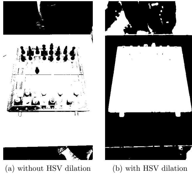
Figure 10: Comparison of the impact of HSV dilation on the thresholding step
