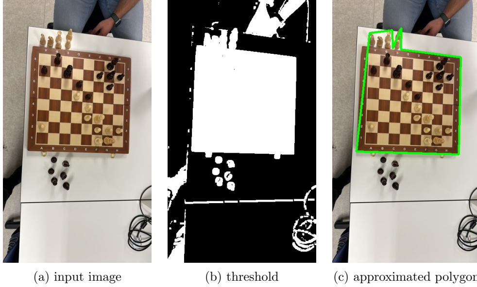
Figure 15: Failure to detect chessboard in image of first dataset due to captured figures standing too close to the edge of the board
