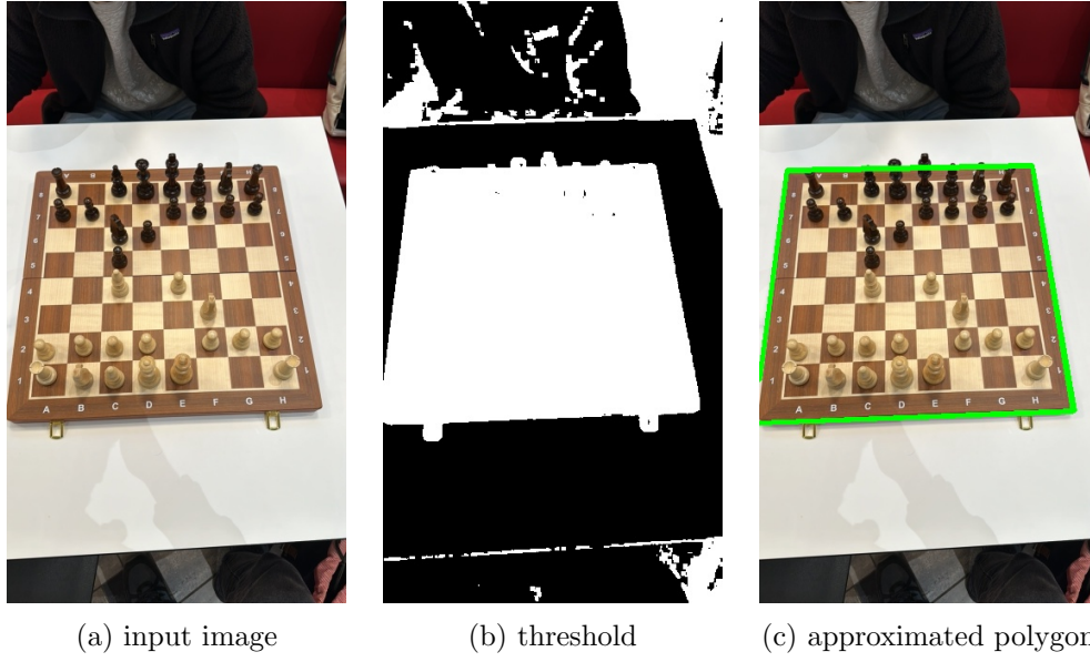
Figure 17: Failure to detect chessboard in image of second dataset due to cut off left bottom corner in input image
