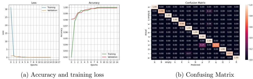
Figure 22: Results of training CNN classifier
